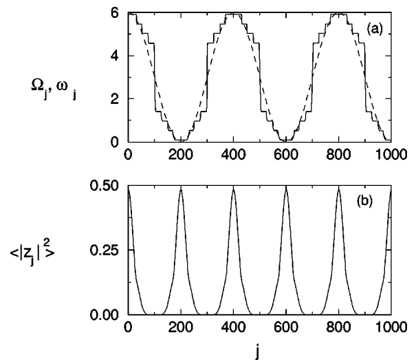
FIG. 1. (a) The dashed line shows the spatial distribution of natural frequencies \omega_j in the model (1). The solid line shows the averaged frequencies of oscillations \Omega_j of the elements of the array (1) for such \omega_j . (b) Spatial profile of time-averaged intensity of oscillations \langle |z_j|^2 \rangle . One can easily see regions of synchronized clusters of oscillations (where the spatial variations of natural frequencies \omega_j are relatively slow—in the vicinity of the extrema of cosinoidal distribution of \omega_j in space) and regions of oscillator death with infinitely small amplitude of oscillations (where the gradient of \omega_j is relatively large).
