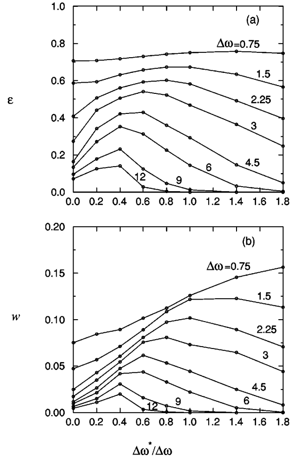
FIG. 5. Dependences of “coherent” (a) and “incoherent” (b) energies \varepsilon and w on the relative level of disorder \Delta\omega^*/\Delta\omega introduced by the rule (4) for different values of linear frequency trend \Delta\omega .
